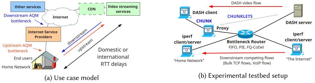
Fig. 1. Our use case model and experimental testbed setup emulating a home network connected to the Internet with AQM enabled at the ISP end and/or home gateway.
