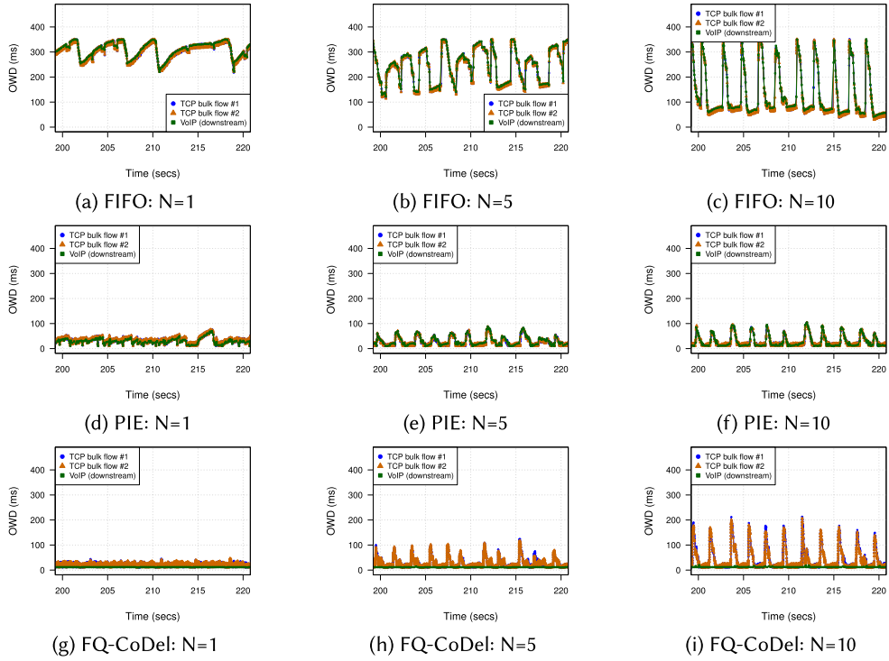
Fig. 7. OWD experienced by TCP bulk flows and downstream VoIP for N=\{1, 5, 10\} and M=2 , in a 20-s window. The VoIP flow is protected and prioritised by FQ-CoDel; hence, it experienced delays that are close to the path's intrinsic OWD (10 ms).
