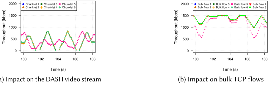
Fig. 13. FQ-CoDel, N=6 , M=8 : Chunklet #5 collides with Bulk Flow #5, resulting in reduced throughput.
