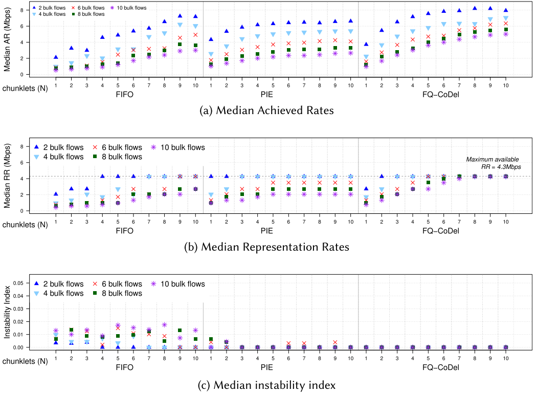
Fig. 4. Median AR, RR, instability index for N=\{1, \dots, 10\} chunklets and M=\{2, 4, 6, 8, 10\} competing bulk TCP flows over {FIFO, PIE, and FQ-CoDel} bottlenecks. All three queue types see benefits of chunklets, but FQ-CoDel provides the best QoE with higher median RRs without any RR oscillations (zero instability index).
