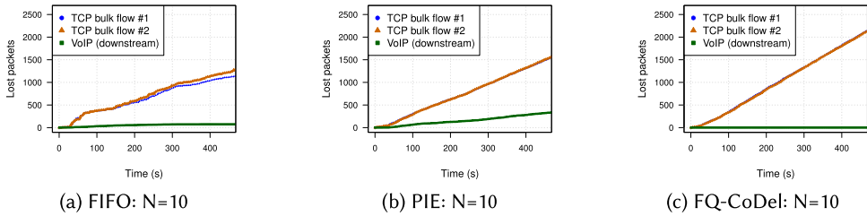
Fig. 8. Cumulative packet losses of TCP bulk flows and downstream VoIP flow when N=10 and M=2 . FQ-CoDel protects and prioritises the low-rate VoIP flow, hence, no VoIP packet losses.
