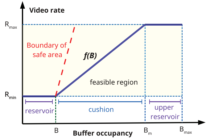
Fig. 6. Buffer-based adaptation rate map (adapted from [86, Fig. 6]).
